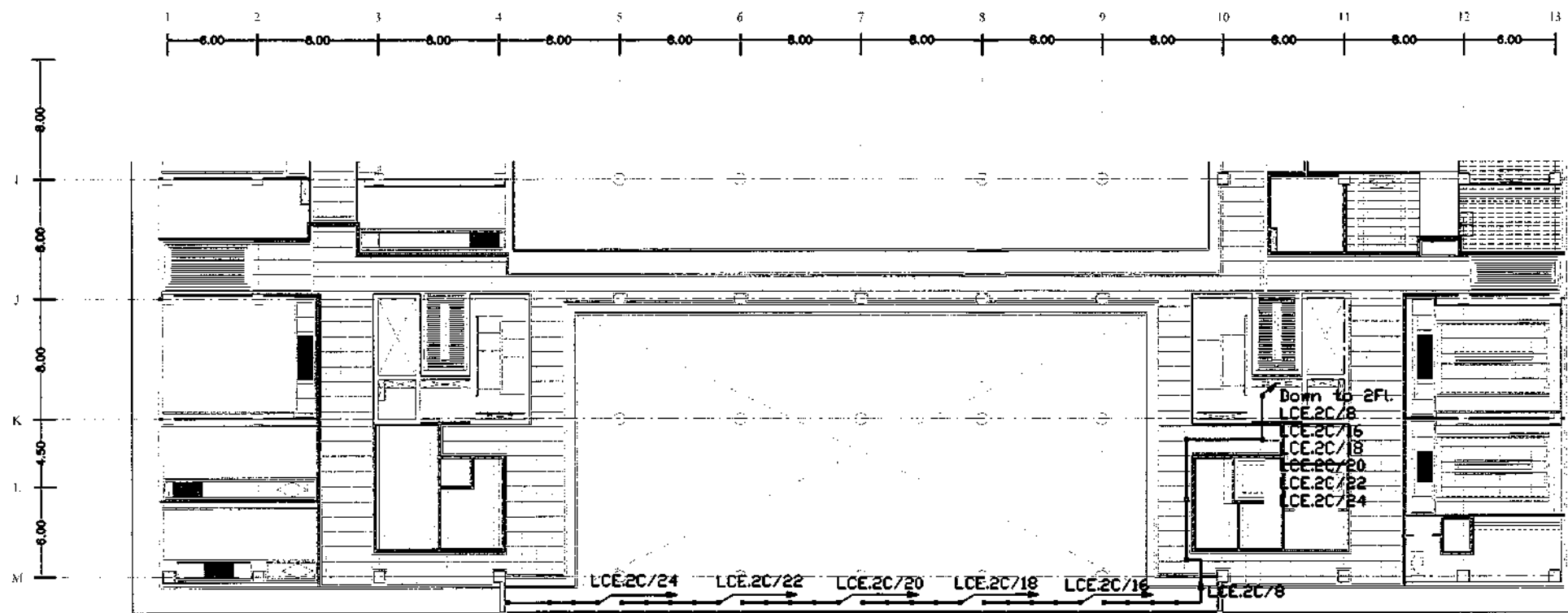
4th FLOOR PLAN
